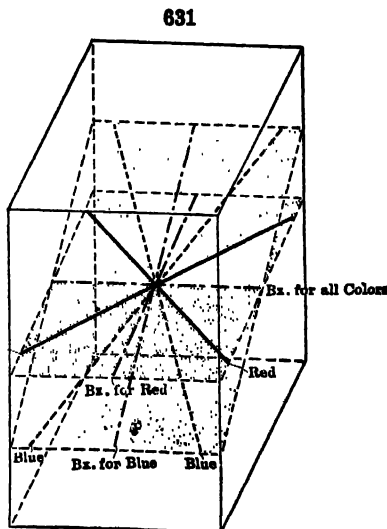
Horizontal Dispersion
